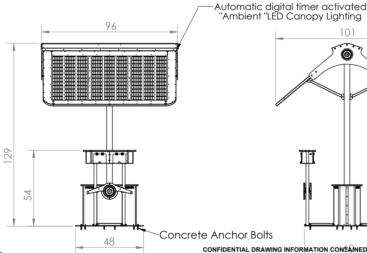
(6) 130 watt Solar Panels
